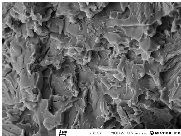
Figure 2. Brittle cleavage mode of fracture, fractured flange.
